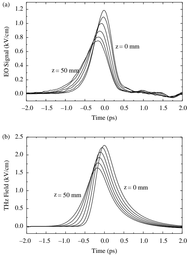
Fig. 2. Temporal field waveforms of a focused THz pulse. The observation position was changed from the focus ( z=0 mm) to 50 mm away from the focus ( z=50 mm) by a step of 10 mm: (a) Experimentally obtained data; (b) Calculated data obtained by simulation assuming Gaussian-beam propagation of each frequency component.
