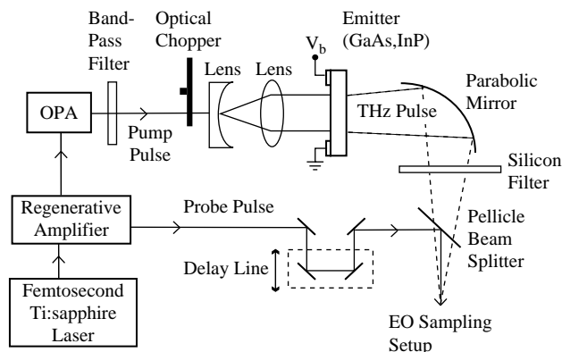
Fig. 6. Schematic of the experimental setup for the THz waveform measurement. OPA is for an optical parametric amplifier.
