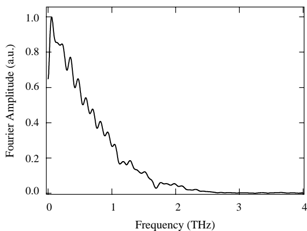
Fig. 4. Typical spectrum of the THz pulses.
